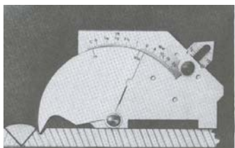
Mordeduras
